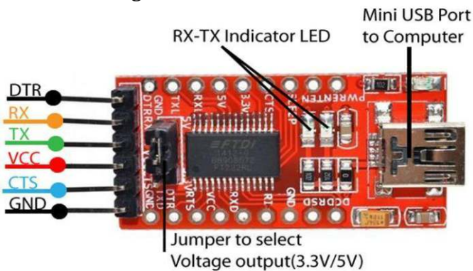
Figure 7: FTDI Programmer Module
